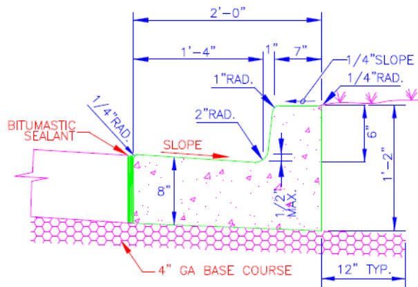
CURB/WITH NORMAL GUTTER
